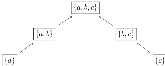
Figure 1.6: The lattice associated with P(X, f) .
