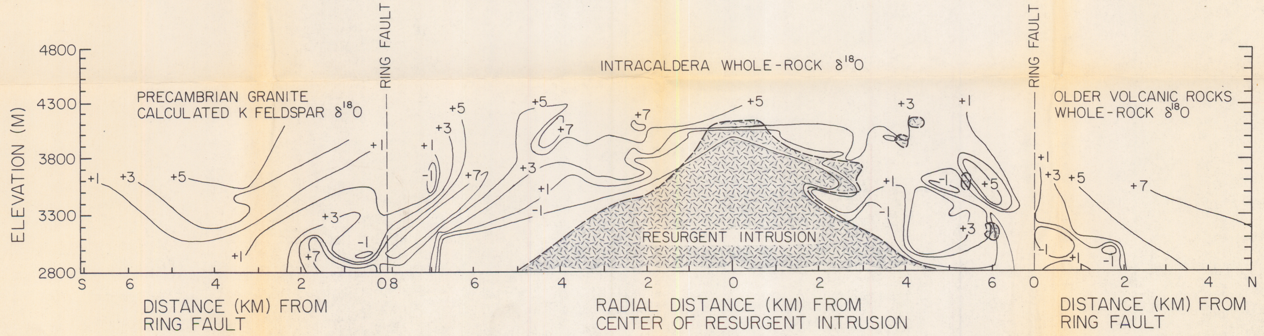
COMPOSITE RADIAL CROSS SECTION OF THE LAKE CITY CALDERA SHOWING \delta^{18}O CONTOURS
