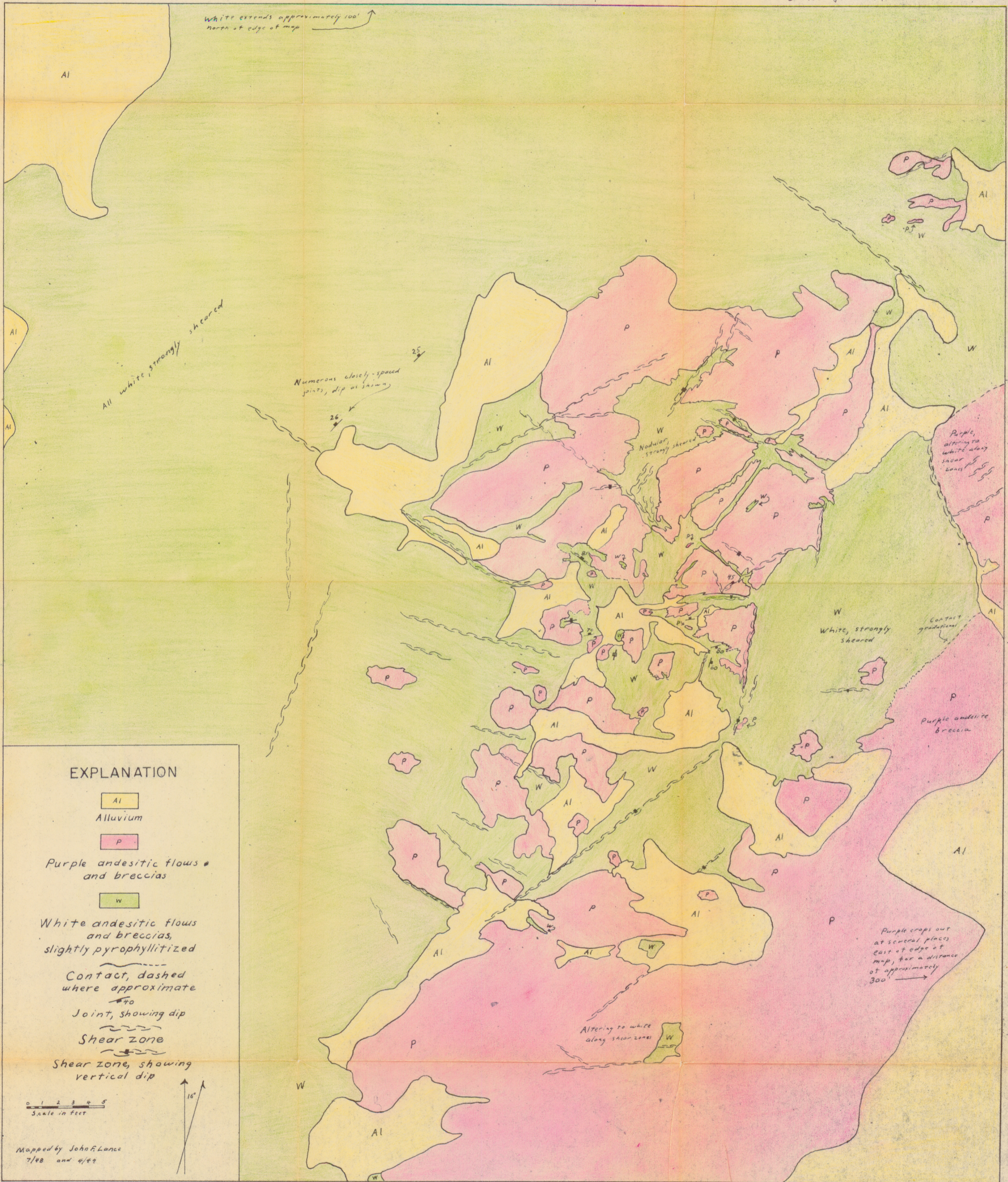
PLATE 3. GEOLOGICAL MAP OF AN AREA NEAR THE PIONEER PYROPHYLLITE DEPOSIT, SAN DIEGO COUNTY, CALIFORNIA
