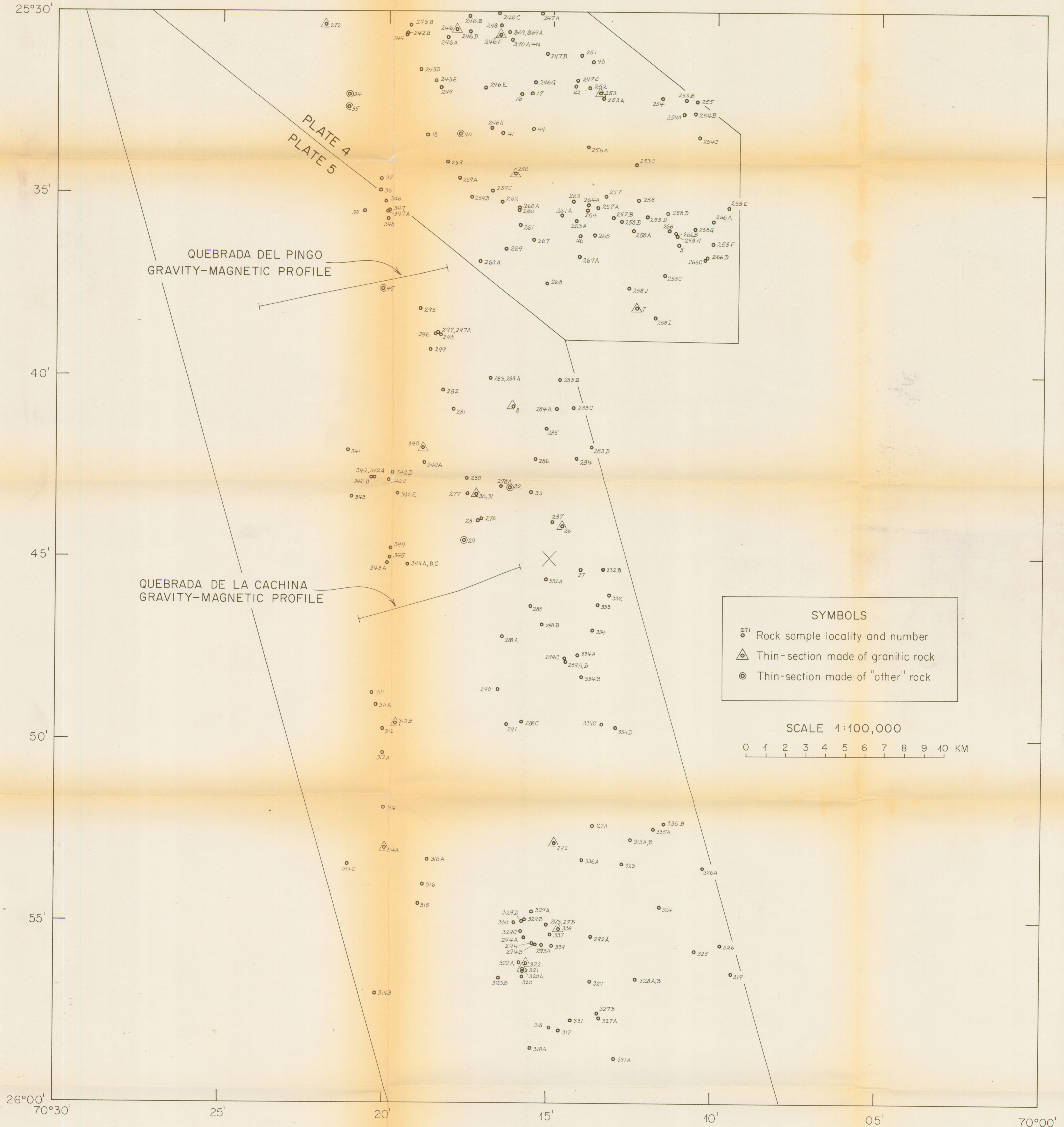
APPENDIX PLATE D. (FOR USE WITH PLATES 4 AND 5.) SAMPLE LOCALITIES FOR ROCKS WHOSE SAMPLE NUMBERS ARE PREFIXED BY "CE". RELATION OF PLATE 5 AND PART OF PLATE 4 TO CERRO DEL PINGO QUADRANGLE (INST. GEOGRÁFICO MILITAR DE CHILE) IS SHOWN.
