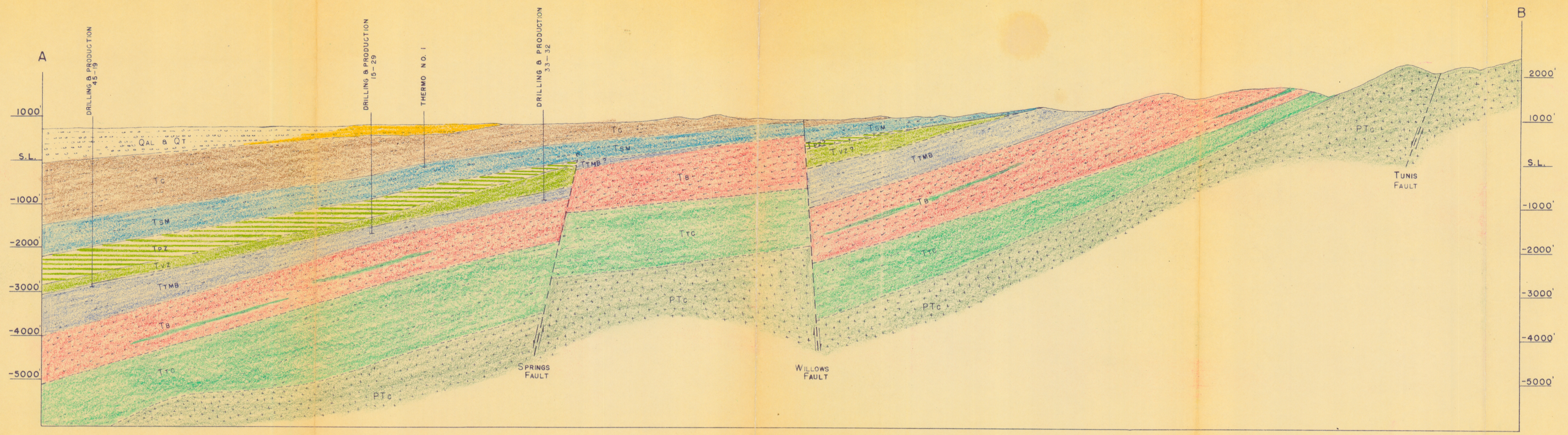
CROSS-SECTION A-B SUBSURFACE GEOLOGY INFERRED FROM ADJACENT WELLS
