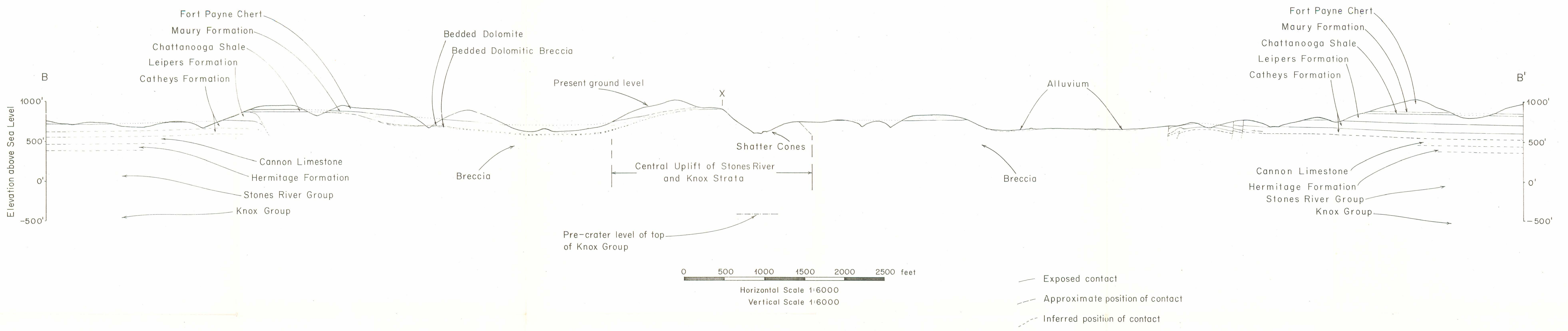
Cross Section B-B' of the Flynn Creek Crater, Tennessee
