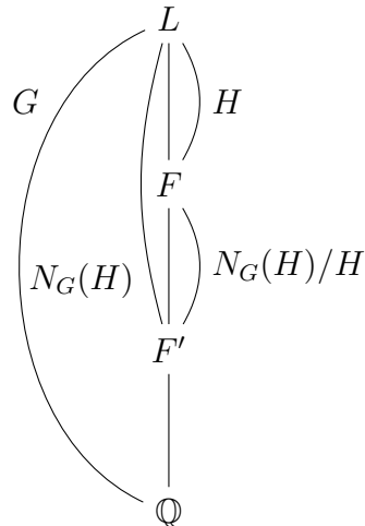
Figure 3.1: The tower of fields and Galois groups. Denote by L the splitting field of \tilde{f} over \mathbb{Q} and regard F as a subfield of L .
