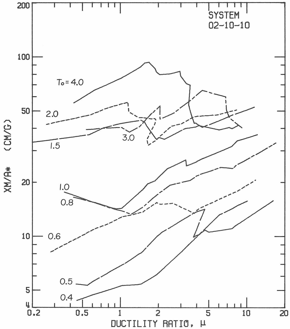
Figure 4.7. Maximum Displacement versus Ductility Ratio for 02-10-10 System and HOL Earthquake.
