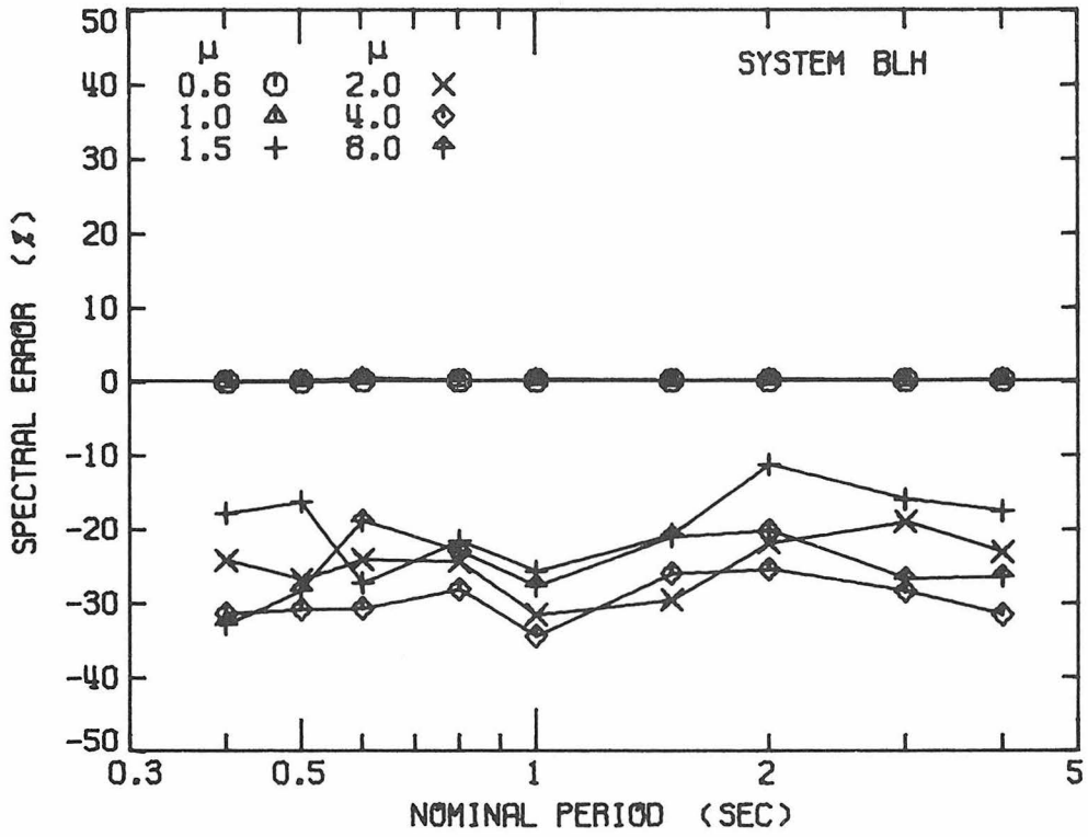
Figure 5.8a. Spectral Error - Average Spectra.
