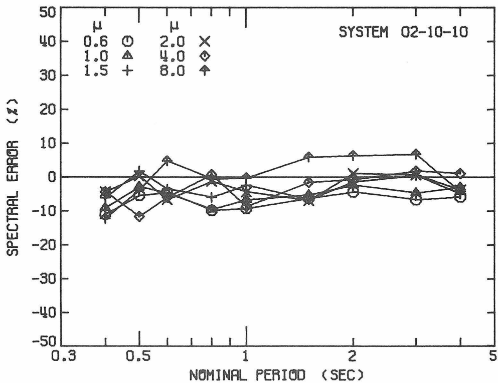
Figure 5.9b. Spectral Error - Average Spectra.
