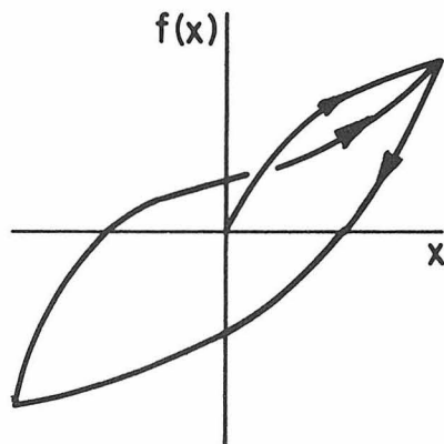
d- Deteriorating
