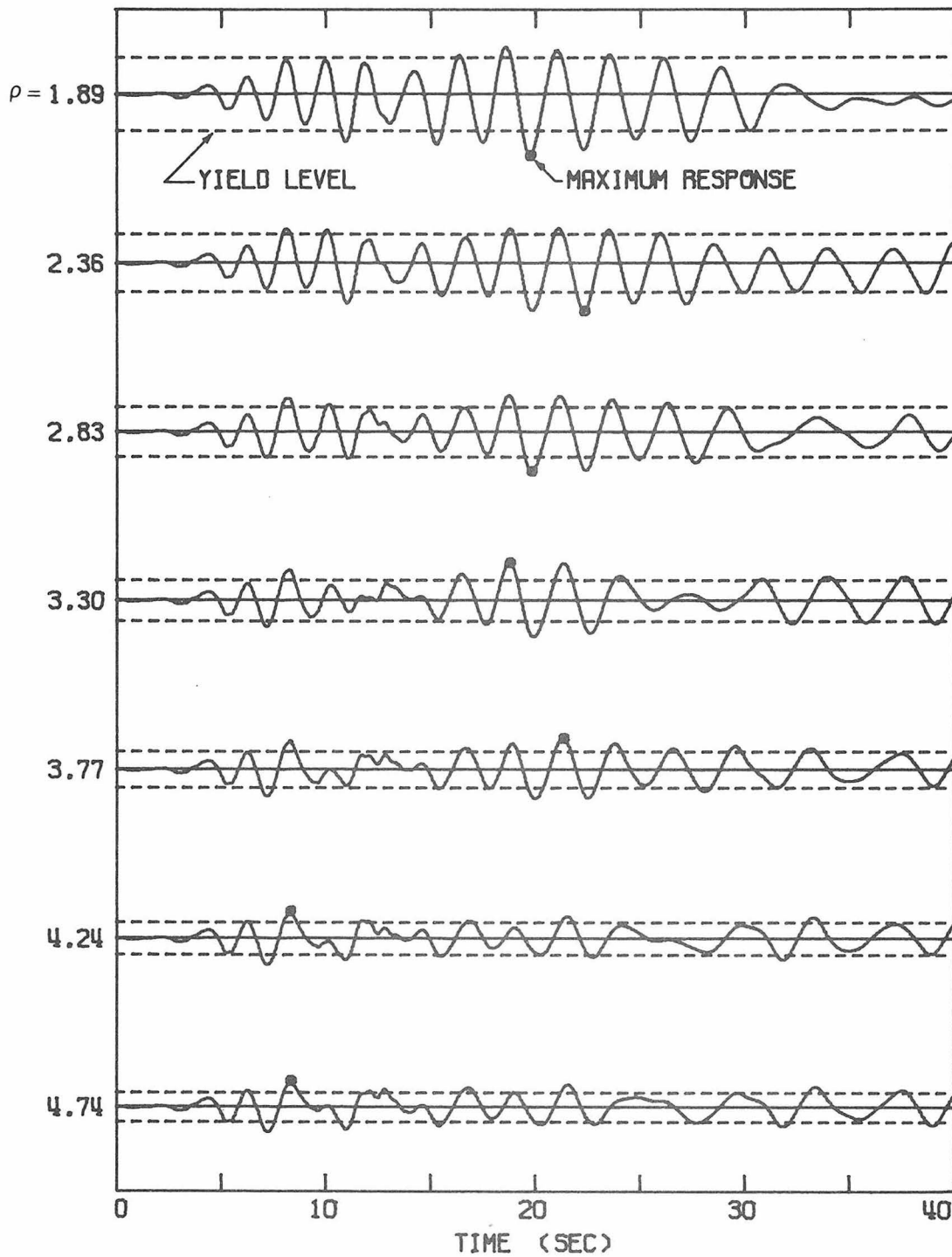
Figure 4.10. Time Histories of Response for HOL Earthquake, 02-10-00 System with T_0 = 2.0 seconds. Vertical Scale is the same in all seven cases.
