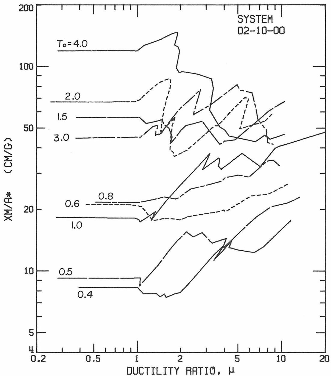
Figure 4.8. Maximum Displacement versus Ductility Ratio for 02-10-00 System and HOL Earthquake.
