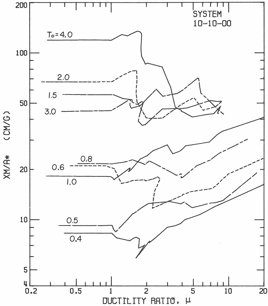
Figure 4.9. Maximum Displacement versus Ductility Ratio for 10-10-00 System and HOL Earthquake.
