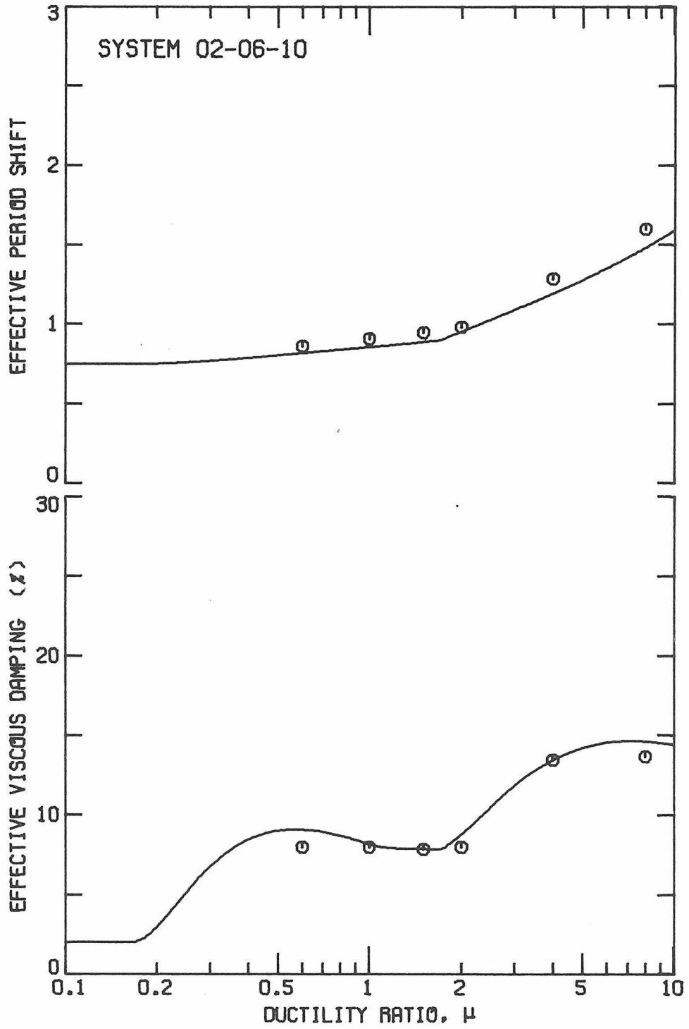
Figure 5.3. ASE Method Linear System Parameters for the 02-06-10 System with \alpha = 5\% and \zeta_0 = 2\% .
