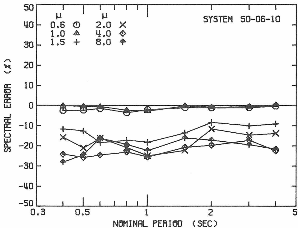
Figure 5.9a. Spectral Error - Average Spectra.
