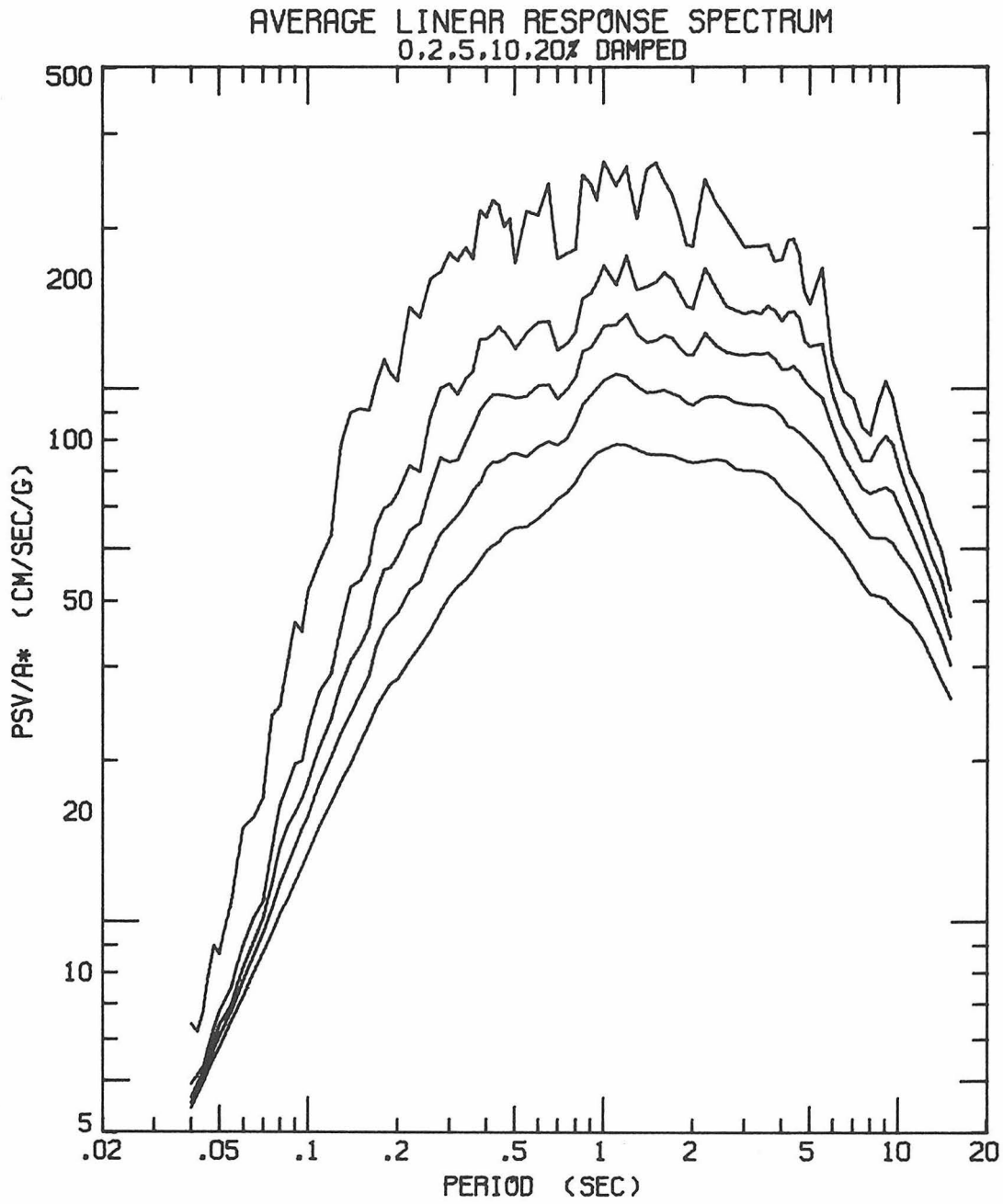
Figure 4.2. Average Spectrum for the Twelve Earthquakes in the Ensemble.
