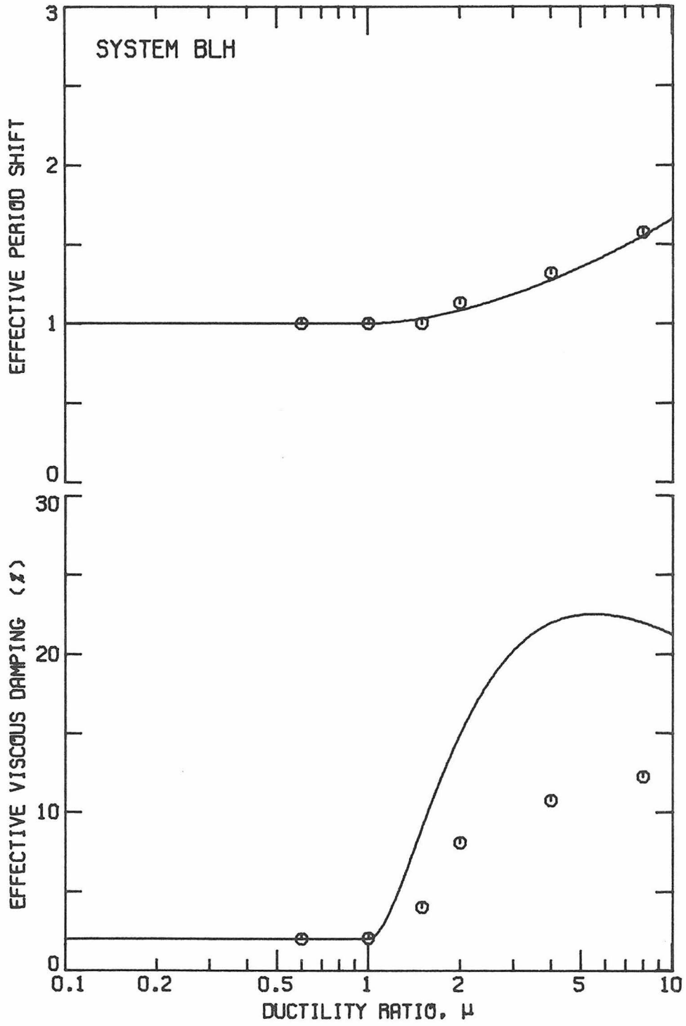
Figure 5.2. ASE Method Linear System Parameters for the BLH System with \alpha = 5\% and \zeta_0 = 2\% .
