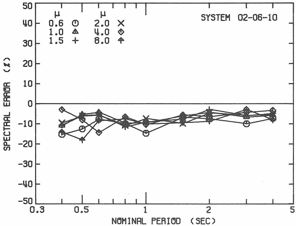
Figure 5.8b. Spectral Error - Average Spectra.
