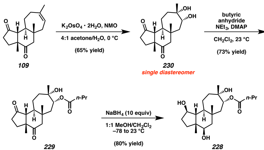
Scheme A10.1 Synthesis of diversification intermediate 228 through a syn-dihydroxylation pathway
