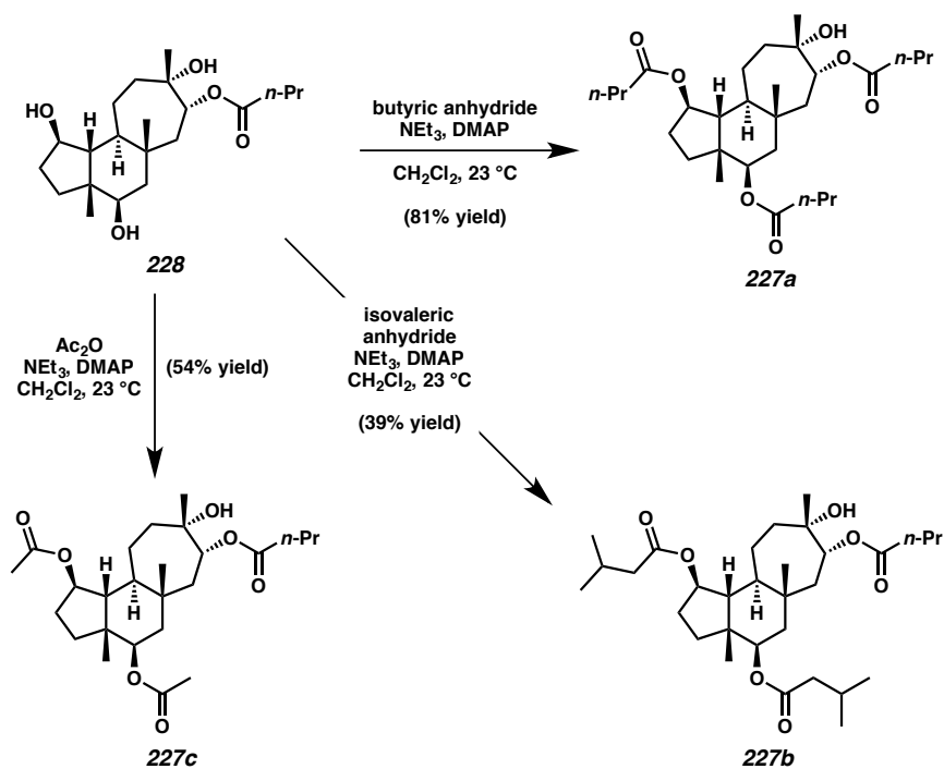
Scheme A10.2 Synthesis of cyanthiwigin–gagunin hybrids 227a–c from common intermediate 228
