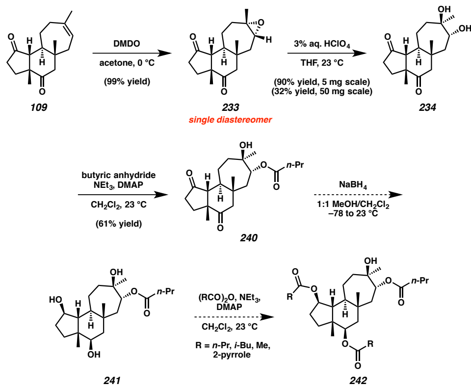
Scheme A10.3 Progress toward hybrids 242 through an anti-dihydroxylation route
