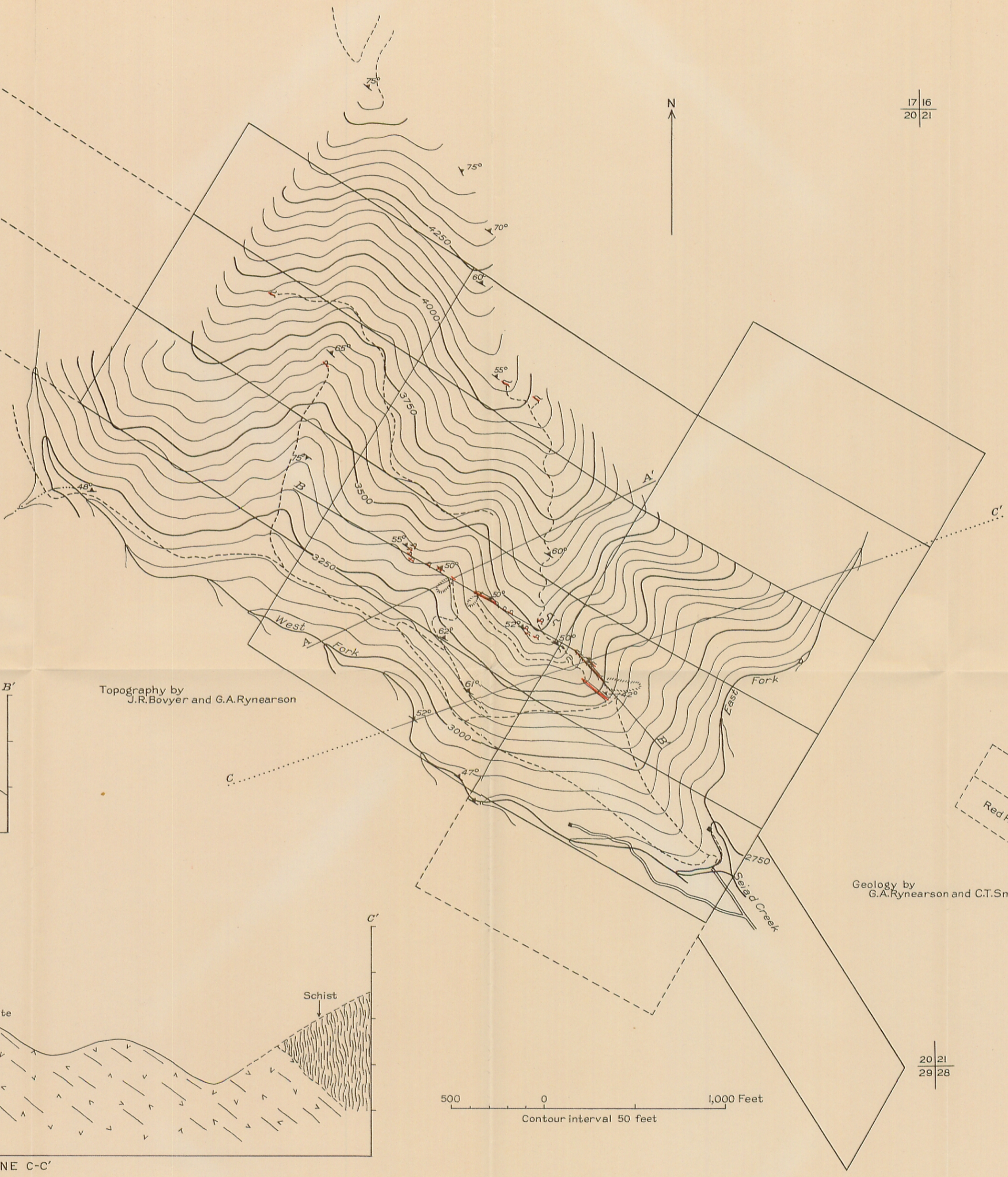
MAP AND SECTIONS OF THE SEIAD CREEK CHROMITE DEPOSIT, SISKIYOU COUNTY, CALIFORNIA
