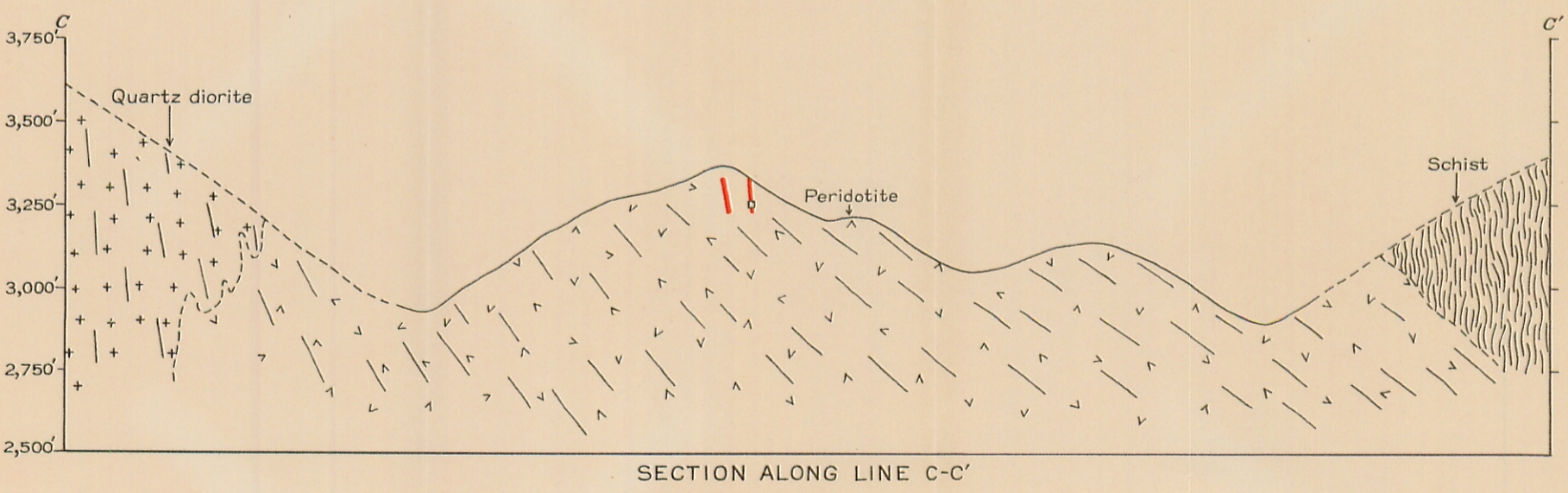
MAP AND SECTIONS OF THE SEIAD CREEK CHROMITE DEPOSIT, SISKIYOU COUNTY, CALIFORNIA
